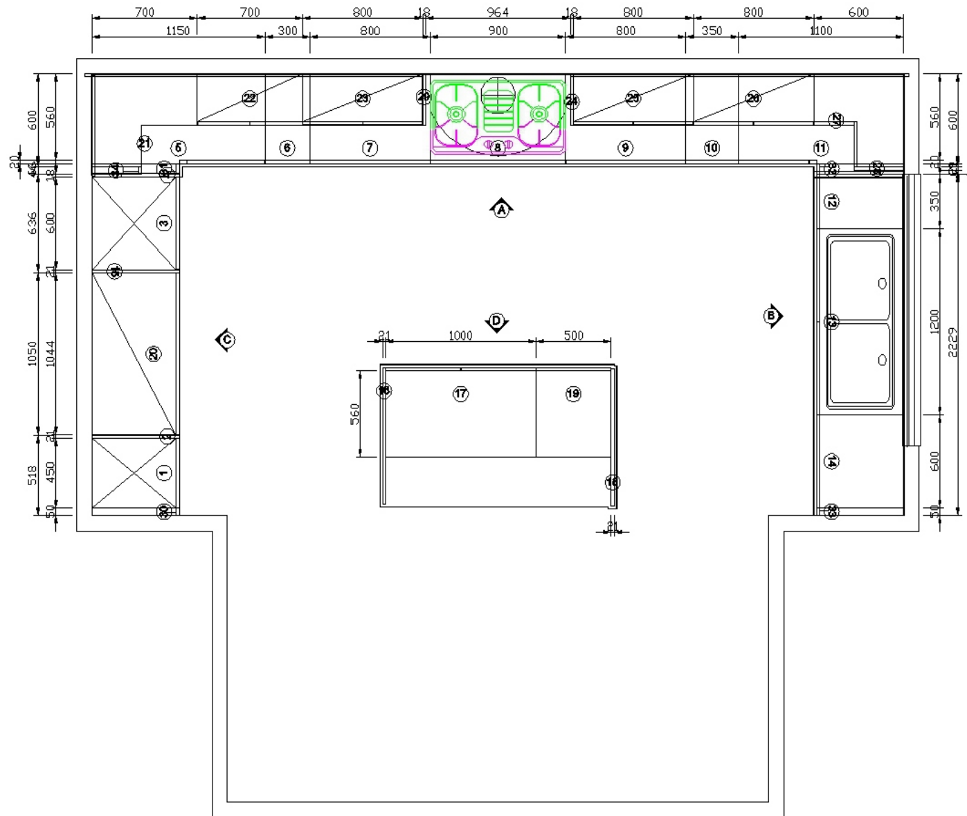
Plan drawing
