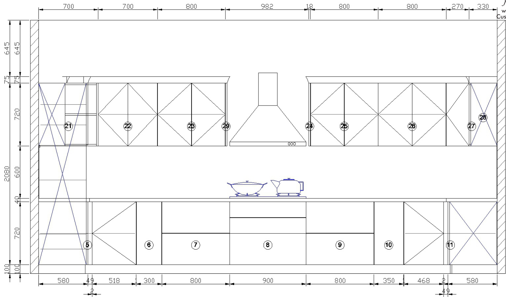
A View elevation drawing
